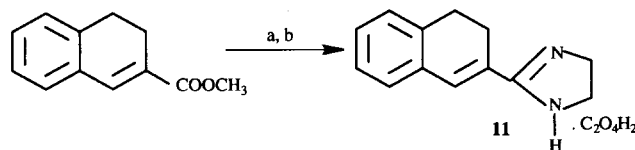
Scheme 4. Reagents and conditions: (a) H 2 NCH 2 CH 2 NH 2 , 2 M Al(CH 3 ) 3 , 2 N NaOH, 2 N HCl; (b) C 2 O 4 H 2 .
