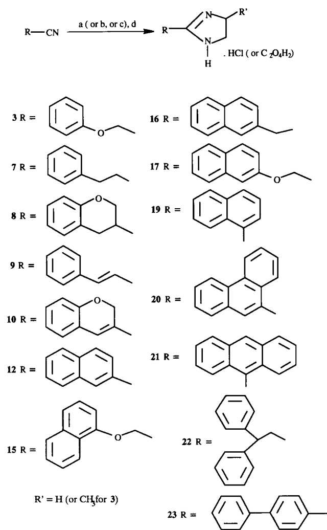
Scheme 1. Reagents and conditions: (a) HCl(g)/CH 3 OH, H 2 NCH 2 CH 2 NH 2 [or H 2 NCH(CH 3 )CH 2 NH 2 ], 2 N NaOH; (b) CH 3 ONa/CH 3 OH, H 2 NCH 2 CH 2 NH 2 , HCl(g)/CH 3 OH, 2 N NaOH; (c) H 2 NCH 2 CH 2 NH 2 .PTSA, 2 N NaOH; (d) 2 N HCl (or C 2 O 4 H 2 ).
