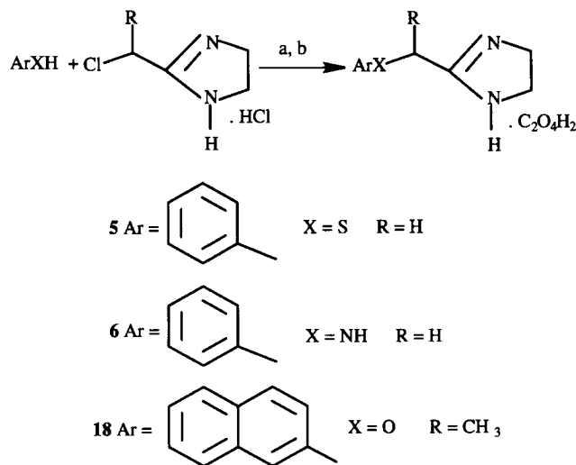
Scheme 2. Reagents and conditions: (a) HCOOH/HCHO, NaOH (pellets); (b) C 2 O 4 H 2 .
