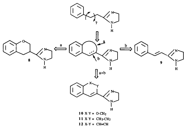
Figure 1. Design strategy to restrict conformation of compound 7 .
