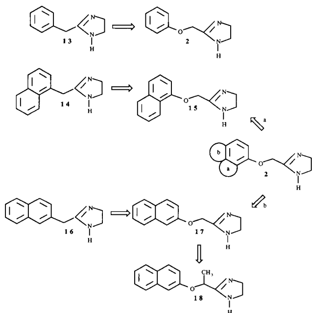
Figure 2. Comparison of tolazoline 13 and compound 2 , and strategy to design compounds 15 , 17 , and 18 .
