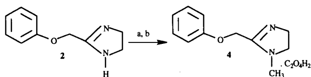
Scheme 2. Reagents and conditions: (a) HCOOH/HCHO, NaOH (pellets); (b) C 2 O 4 H 2 .
